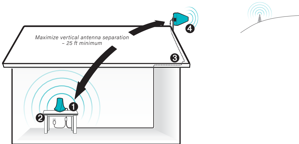
Installation overview
